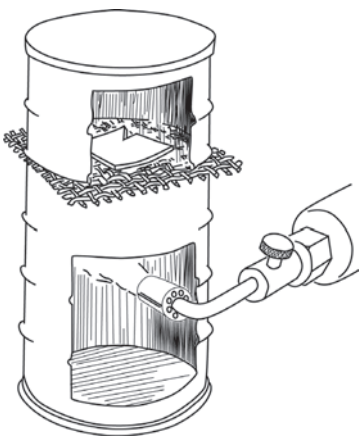
Image 2: Torch kiln
